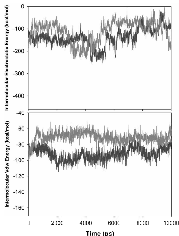
Figure 9. Intermolecular electrostatic (a) and vdw energy (b) between outermost fA \beta sheaf. Red line indicates fA \beta fibrils with myricetin and blue line indicates fA \beta fibrils alone.
