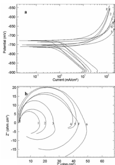
[(F) 0.00 (1) 1.0 \times 10^{-4} (2) 2.5 \times 10^{-3} (3) 1.0 \times 10^{-2} (4) 2.5 \times 10^{-2} (5) 3.0 \times 10^{-2} (6) 5.0 \times 10^{-2} ] M
