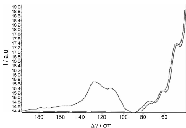
Figure 4. The Raman spectra of MMI-disulfide (---) and MMI-disulfide:iodine (1:1) complex, (\text{MMI-disulfide})\text{I}_3^- (—).
