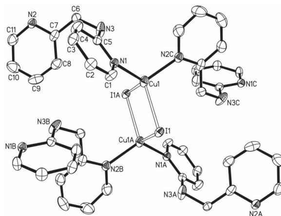
Figure 1. Ortep representation showing the coordination environments of metal centers in 1 , [\text{Cu}(\text{L})]_n . Hydrogen atoms and disorder parts are omitted for clarity. [Symmetric codes: A) -x+1, -y+1, -z+1 ; B) x, -y+0.5, z+0.5 ; C) -x+1, y+0.5, -z+0.5 ]
