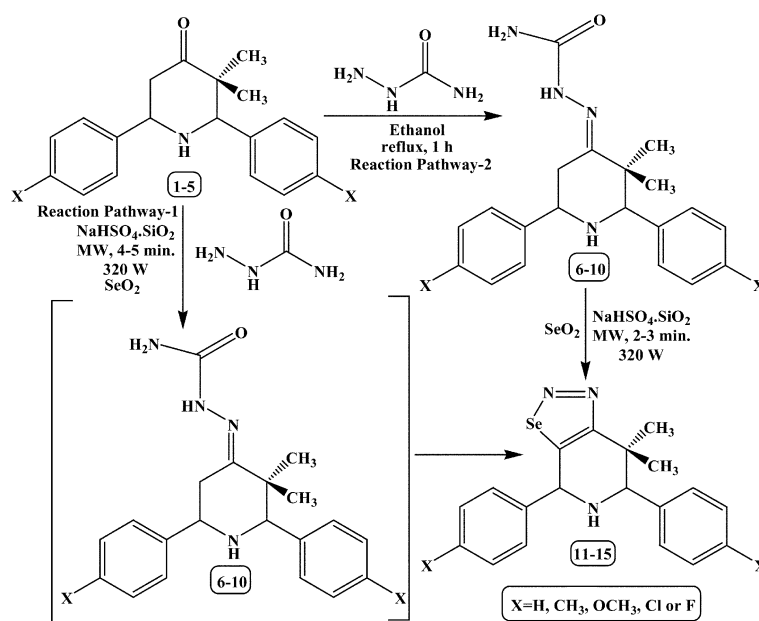
Scheme 1. One-pot synthesis of 5,7-diaryl-4,4-dimethyl-4,5,6,7-tetrahydropyridino[3,4-d]-1,2,3-selenadiazoles.
