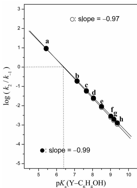
Figure 3. Plots of \log k_2/k_{-1} vs pK_a of the conjugate acids of the leaving aryloxides for reactions of 5a-h (○) and 6a-h (●) with piperidine in 80 mol % H_2O /20 mol % DMSO at 25.0 \pm 0.1 °C. The identity of points is given in Table 2.
