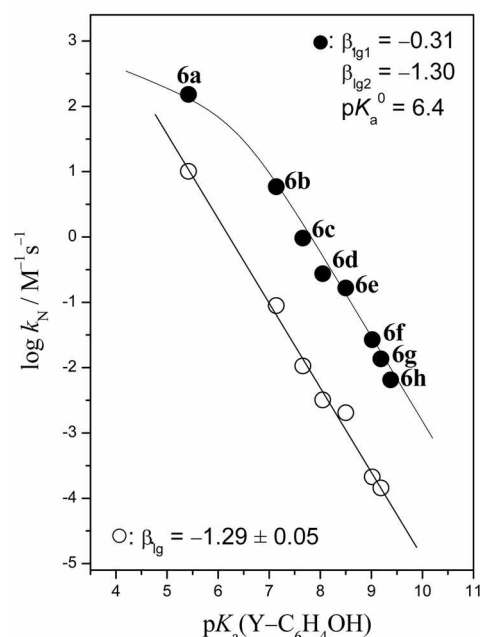
Figure 1. Bronsted-type plots for reactions of 6a-h with morpholine (○) and piperidine (●) in 80 mol % H 2 O/20 mol % DMSO at 25.0 \pm 0.1 ^\circ\text{C} . The identity of points is given in Table 1.
