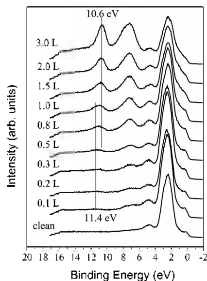
Figure 5. Valence band spectra obtained after exposing W(110) to various amounts of CO at 120 K. A photon energy of 90 eV was used.
