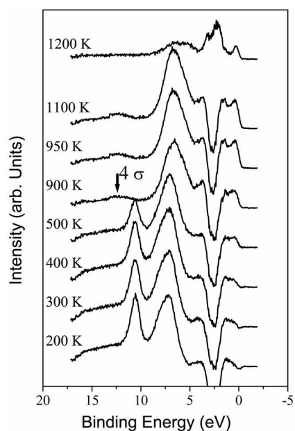
Figure 9. The clean surface spectrum was subtracted from each spectrum in Fig. 7 (difference spectrum). The heating temperature of each spectrum is denoted in the.
