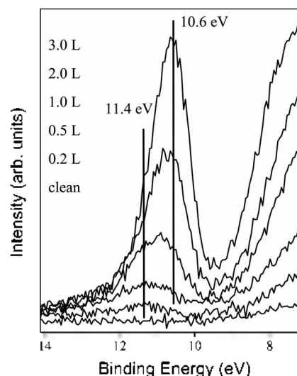
Figure 6. A magnified view of some spectra in Fig. 5 is shown in order to clearly see the evolution of the 4\sigma state as a function of CO exposure.
