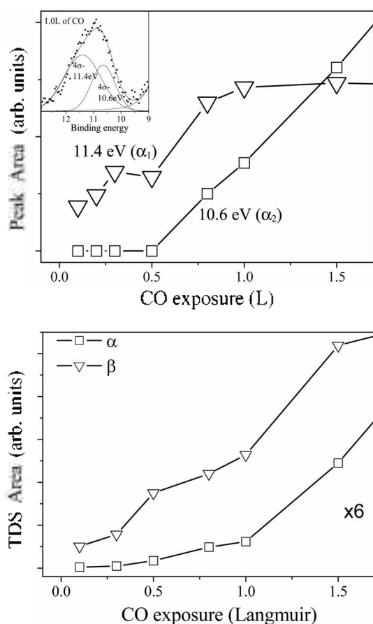
Figure 7. Top: Each spectrum in Fig. 5 was fitted by four Gaussian functions, two of them for the 1\pi + 5\sigma state, and the other two for the 4\sigma state, and the relative intensity ratios of the two different 4\sigma states are summarized. In the inset, a magnified view of a fitted valence band spectrum is shown as a representative example, which was taken after a CO exposure of 1.0 L. Bottom: the relative intensity ratios of the \alpha - and \beta -CO in the TDS spectra in Fig. 1 are summarized.
