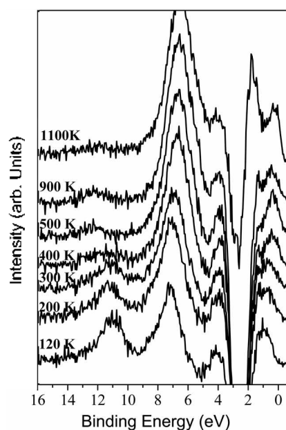
Figure 10. Difference spectra of valence band spectra collected after exposing W(110) to 0.8 L of CO at 120 K followed by stepwise heating. The heating temperature of each spectrum is given in the figure.
