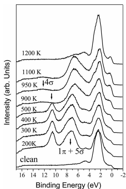
Figure 8. W(110) was exposed to 3.0 L of CO at 120 K and the valence band spectra were collected after stepwise heating. The heating temperature for each spectrum is given in the figure.
