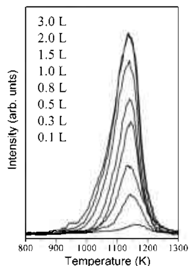
Figure 2. Thermal Desorption Spectra of CO obtained after exposing W(110) to various amounts of CO at 900 K. The heating rate was 6 K/s.
