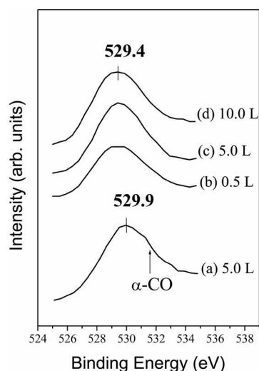
Figure 3. (a) O 1s spectra after exposing W(110) to 5.0 L of CO at room temperature. Synchrotron radiation with a photon energy of 770 eV was used. (b-d) After CO exposure at room temperature, the samples were heated to 900 K and then the O 1s spectra were collected. The CO doses are given in the figure.
