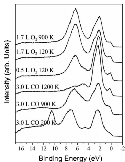
Figure 11. Valence band spectra collected after exposing W(110) to various amounts of CO and O 2 at different temperatures. The details of the gas exposure and temperature are given in the figure.
