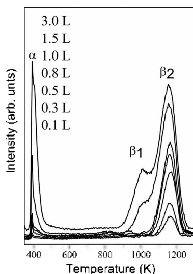
Figure 1. Thermal Desorption Spectra of CO obtained after exposing W(110) to various amounts of CO at room temperature. The heating rate was 6 K/s.
