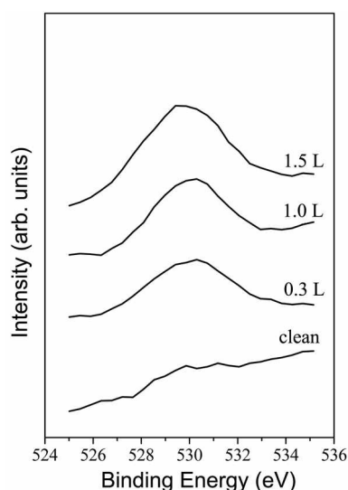
Figure 4. O 1s spectra taken after exposing W(110) to various amounts of O 2 , followed by heating to 1500 K. A photon energy of 770 eV was used.
