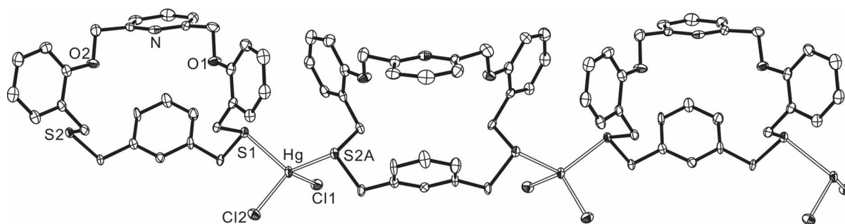
Figure 3. Crystal structure of \{[\text{Hg}(\text{L}^2)\text{Cl}_2]\text{CH}_3\text{OH}\}_n , 2 . Hydrogen atoms and solvent molecules are omitted. Selected bond lengths (Å) and bond angles ( ^\circ ): Hg-S1 2.581(3), Hg-S2A 2.549(3), Hg-Cl1 2.448(3), Hg-Cl2 2.437(3), S1-Hg-S2A 121.9(1), S1-Hg-Cl2 100.6(1), S2A-Hg-Cl1 105.2(1), Cl1-Hg-Cl2 119.4(1), S1-Hg-Cl1 101.7(1), Cl2-Hg-S2A 109.0(1). Symmetry codes A: x+1/2 , -y+3/2 , z-1/2 .
