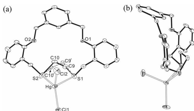
Figure 2. Crystal structure of [\text{Hg}(\text{L}^1)\text{Cl}_2] , 1 . (a) front view and (b) side view. Hydrogen atoms are omitted. Selected bond lengths (Å), bond angles ( ^\circ ) and torsion angles ( ^\circ ): Hg-S1 2.818(1), Hg-S2 2.504(1), Hg-Cl1 2.381(1), Hg-Cl2 2.454(1), S1-Hg-S2 80.3(1), S1-Hg-Cl1 112.2(1), S1-Hg-Cl2 99.9(1), Cl1-Hg-Cl2 114.0(1), S2-Hg-Cl2 109.0(1), S2-Hg-Cl1 131.5(1), S1-C9-C10-S2 -64.9(8), S1-C9'-C10'-S2 73.5(9).
