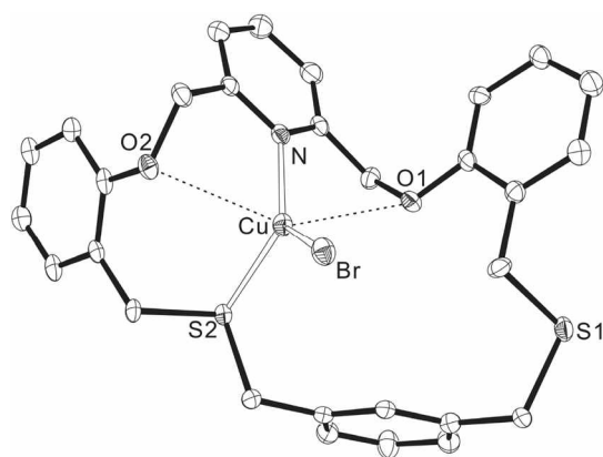
Figure 4. Crystal structure of [\text{Cu}(\text{L}^2)\text{Br}] , 3 . Hydrogen atoms are omitted. Selected bond lengths (Å), bond angles ( ^\circ ), torsion angles ( ^\circ ) and interatomic distances (Å): Cu-N 1.999(3), Cu-S2 2.298(1), Cu-Br 2.348(1), N-Cu-S2 115.9(1), N-Cu-Br 129.6(1), S2-Cu-Br 113.4(1), O1-C1-C29-N -44.6(4), O2-C25-C24-N 55.5(3), Cu...O1 2.850(2), Cu...O2 2.716(2).
