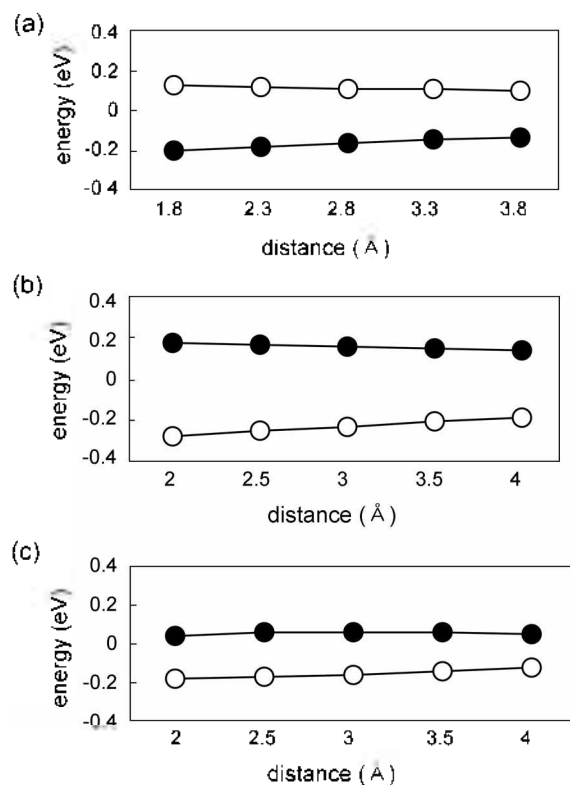
Figure 7.1. 22BPY-Au(111) interaction energy \Delta E_s , calculated as a function of the distance between the model surface of point charges \delta and the closest atoms of the 22BPY cis configuration to the surface: (a) a 22BPY cis configuration is perpendicular with the N atoms facing away from the surface, (b) a 22BPY cis configuration is perpendicular with the N atoms facing the surface, and (c) 22BPY cis configuration lies flat and parallel to the surface. The \Delta E_s values for \delta = 0.05 are represented by filled circles, and those for \delta = +0.05 are indicated by empty circles.
