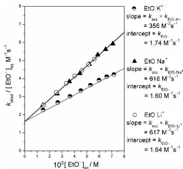
Figure 3. Plots illustrating dissection of k_{obsd} into rate constants due to dissociated and ion-paired ethoxides for reactions of 5-nitro-8-quinoyl benzoate ( 5 ) with EtO^-M^+ in anhydrous EtOH at 25.0 \pm 0.1 °C.
