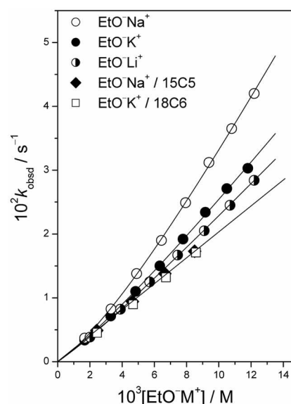
Figure 1. Plots of k_{obsd} vs. [EtO^-M^+] for reactions of 5-nitro-8-quinolyl benzoate ( 5 ) with EtO^-Na^+ ( \circ ), EtO^-K^+ ( \bullet ), EtO^-Li^+ ( \ominus ), EtO^-Na^+/15C5 ( \blacklozenge ; [15C5]/[EtO^-Na^+] = 5.0 ), and EtO^-K^+/18C6 ( \square ; [18C6]/[EtO^-K^+] = 5.0 ) in anhydrous EtOH at 25.0 \pm 0.1 °C.
