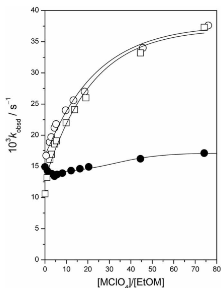
Figure 2. Plots showing effect of added salts ( MClO_4^- ) on the reactivity for reactions of 5-nitro-8-quinoyl benzoate ( 5 ) with EtO^-M^+ in anhydrous EtOH at 25.0 \pm 0.1 °C. EtO^-Na^+ + Na^+ClO_4^- ( \circ ), EtO^-Li^+ + Na^+ClO_4^- ( \square ), EtO^-Na^+ + Li^+ClO_4^- ( \bullet ). [EtO^-Na^+] = 5.08 \times 10^{-3} M, [EtO^-Li^+] = 4.93 \times 10^{-3} M.
