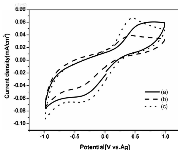
Figure 4. Cyclic voltammograms obtained in a 1 M \text{LiClO}_4 propylene carbonate solution at a scan rate of 10 mV/s. The working electrodes are composed of the \text{V}_2\text{O}_5 nanomaterials (75%), carbon (20%), and ethylene cellulose (5%). Film electrodes were prepared to contain the \text{V}_2\text{O}_5 nanomaterial of 2.5 \text{mg}/\text{cm}^2 . The \text{V}_2\text{O}_5 nanomaterials are obtained upon calcination (at 400 ^\circ\text{C} ) of: (a) sample 1, (b) sample 2, and (c) sample 3.
