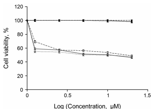
Figure 2. Dark (black figure: ▲, ●, ■) and phototoxicity (white figure: △, ○, □) of PIP (line-triangle-line), IMI (dot-circle-dot) and control starting material HPPH (dash-square-dash) toward A549 cells using 2 J cm^{-2} dose light after 24 h incubation time.
