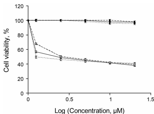
Figure 3. Dark (black figure: ▲, ●, ■) and phototoxicity (white figure: △, ○, □) of PIP (line-triangle-line), IMI (dot-circle-dot) and control starting material HPPH (dash-square-dash) toward A549 cells using 2 J cm^{-2} dose light after 48 h incubation time.
