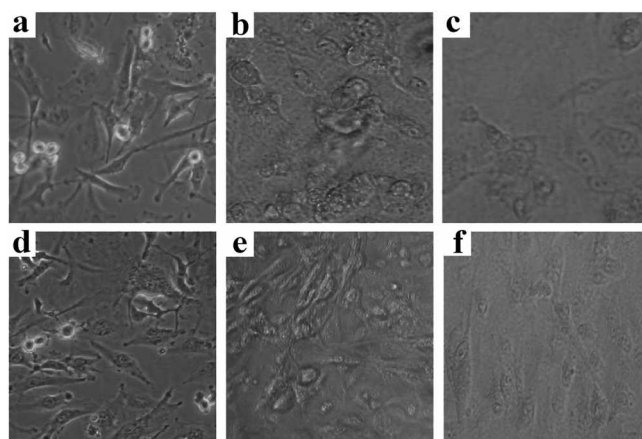
Figure 4. Optical image of morphological changes induced by PIP (b and c) and IMI (e and f) for 24 and 48 h respectively after irradiation compared with control (a and d) at 2.5 \times 10^{-6} M concentration.
