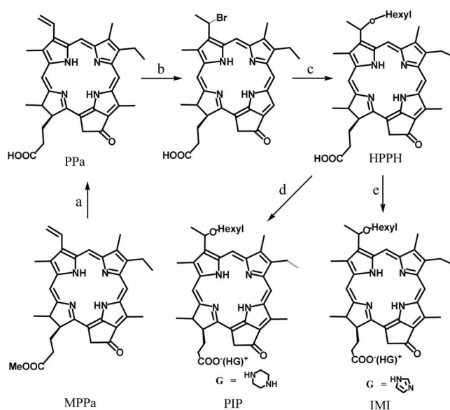
Figure 1. Synthetic pathways of complexes of HPPH with piperazine (PIP) and imidazole (IMI). Reagents: a) KOH, MeOH/THF; b) HBr/ \Delta COH; c) Hexanol/ K_2CO_3/CH_2Cl_2 ; d) piperazine/MeOH/MC; e) imidazole/MeOH/MC.
