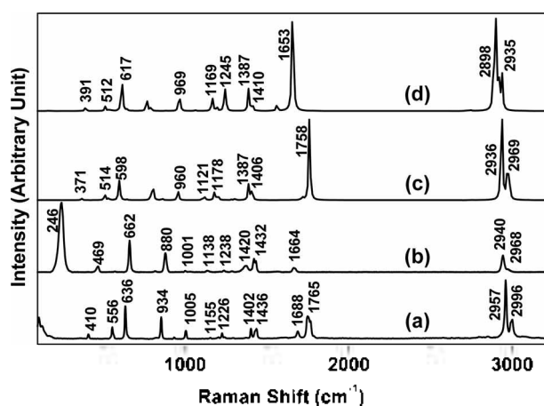
Figure 4. OR spectrum of SI in (a) neat solid state and SERS spectrum of (b) \sim 10^{-3} M SI in aqueous silver nanocolloids at pH \sim 8 in 100\text{--}3250\text{ cm}^{-1} . Simulated spectra of (c) neutral and (d) anionic states of SI from the DFT calculation. Peak intensities are normalized for a better comparison.
