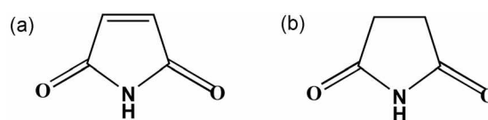
Figure 1. Structures of (a) maleimide (MI) and (b) succinimide (SI).
