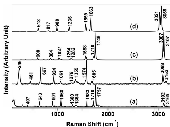
Figure 2. OR spectrum of MI in (a) neat solid state and SERS spectrum of (b) \sim 10^{-3} M MI in aqueous silver nanocolloids at pH \sim 8 in 100 – 3250 \text{cm}^{-1} . Simulated spectra of (c) neutral and (d) anionic states of MI from the DFT calculation. Peak intensities are normalized for a better comparison.
