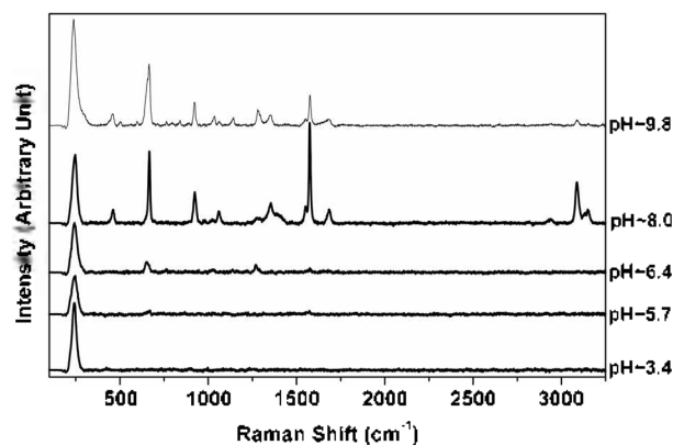
Figure 3. pH-dependent SERS spectra in \sim 10^{-3} M MI in aqueous silver nanocolloids at various pH values.
