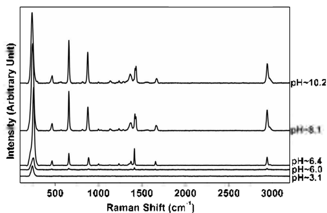
Figure 5. pH-dependent SERS spectra in \sim 10^{-3} M SI in aqueous silver nanocolloids at various pH values.
