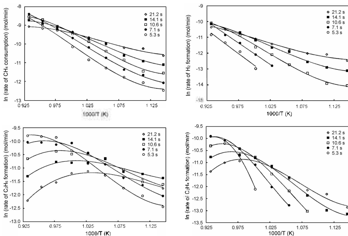
Figure 5. Rates for \text{CH}_4 consumption, \text{H}_2 formation, \text{C}_2\text{H}_6 formation, and \text{C}_2\text{H}_4 formation as a function of reciprocal temperature for the oxidative methane pyrolysis.
