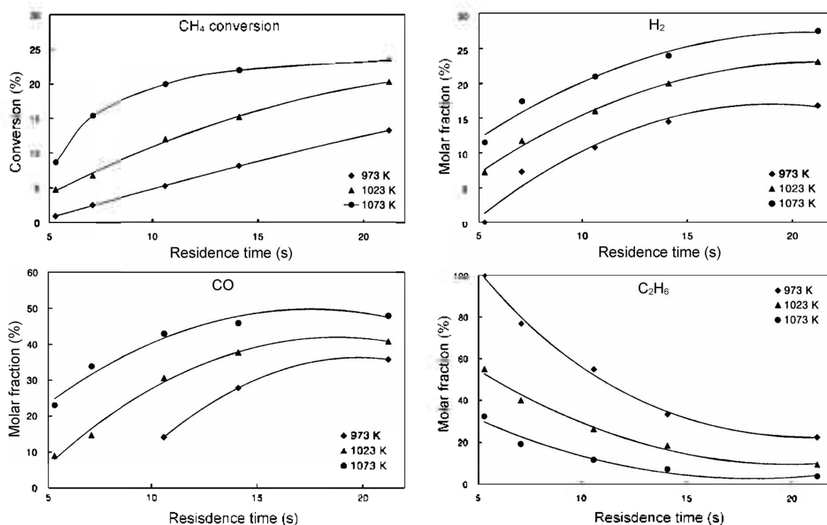
Figure 1. Methane conversion and fractions of products as a function of residence time for the oxidative methane pyrolysis at 973, 1023, and 1073 K.
