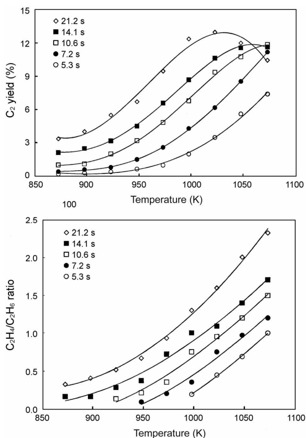
Figure 3. Variations of C_2 yield and C_2H_4/C_2H_6 ratio with temperature at various residence times for the oxidative methane pyrolysis.
