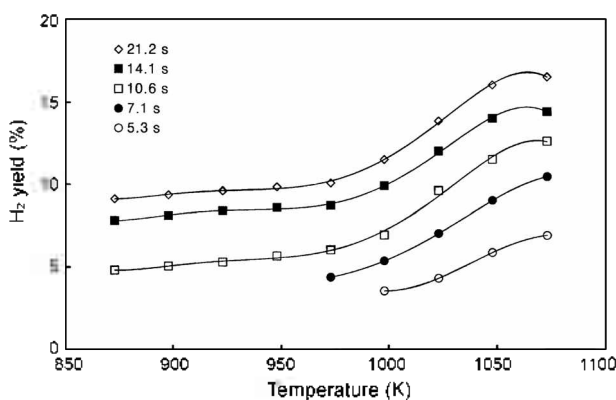
Figure 2. Variation of H 2 yield with temperature at various residence times for the oxidative methane pyrolysis.
