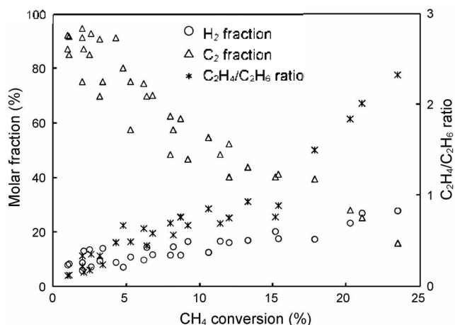
Figure 4. Relationships between C_2 fraction, H_2 fraction, C_2H_4/C_2H_6 ratio, and CH_4 conversion in the oxidative methane pyrolysis.
