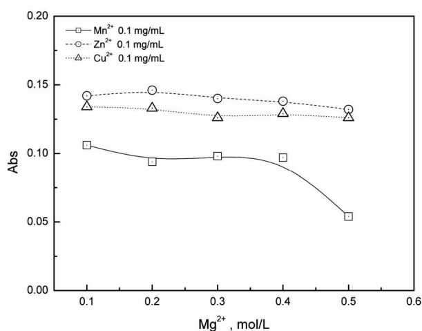
Figure 5. Interference effect of Mg(II) on the extraction of Cu(II), Mn(II) and Zn(II) using salen(NEt 3 ) 2 .
