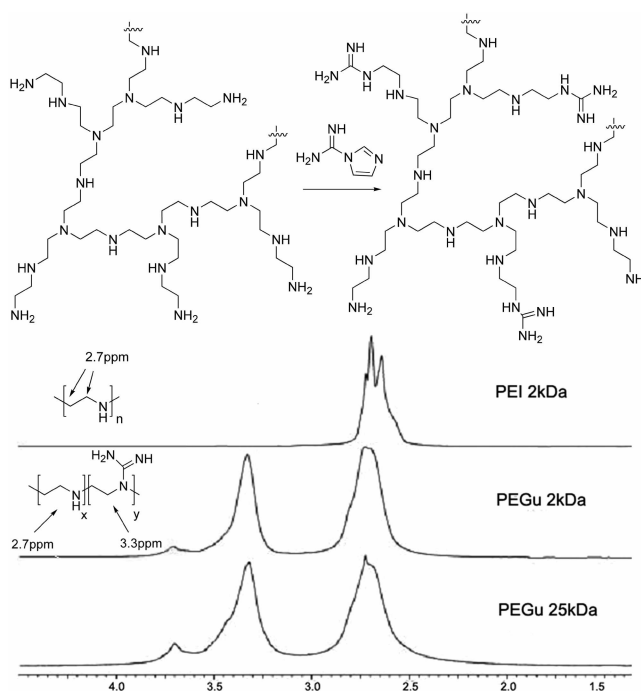
Figure 1. Synthetic scheme of PEGu synthesis and 1 H-NMR spectra of PEI and PEGu.
