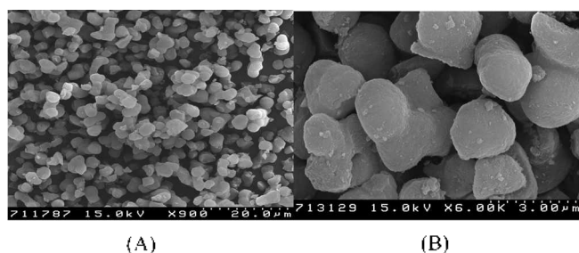
Figure 1. The SEM images of (A) sieved silica monolith particles (3-5 \mu\text{m} ) and (B) the expanded view of A.
