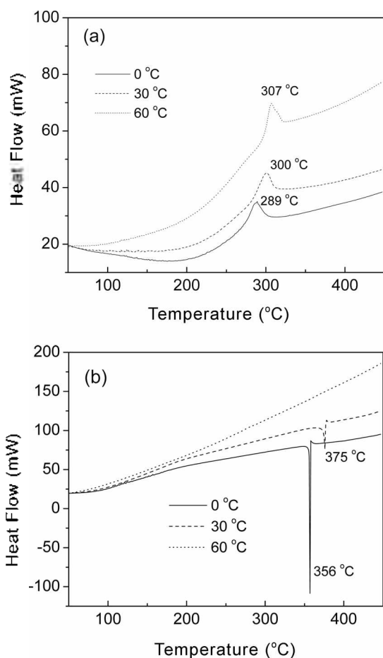
Figure 4. DSC curves of ITO precursors that were prepared at various temperatures and pH 12 (a) and 8 (b) (up endothermic).
