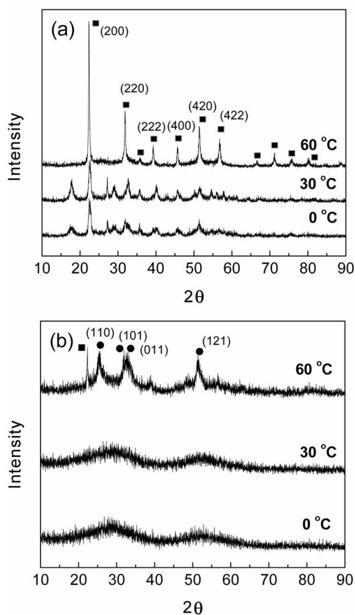
Figure 1. XRD patterns of ITO precursors that were precipitated at various temperatures and pH 12 (a) and 8 (b) without heat treatment. ■ and ● represent XRD peaks of \text{In}(\text{OH})_3 and \text{InOOH} , respectively.
