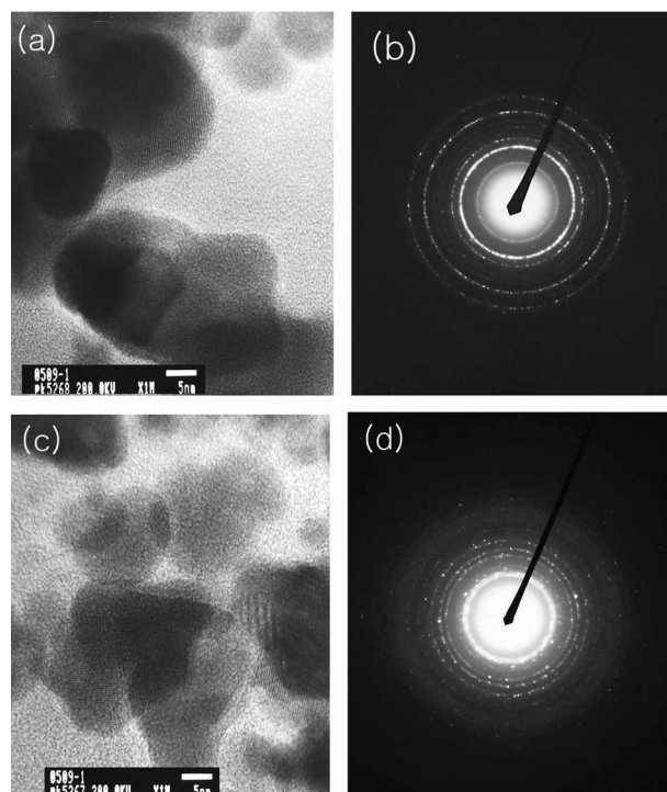
Figure 5. HR-TEM pictures and electron diffraction patterns of ITO nanoparticles that were prepared at pH 8 and 0 °C (a, b) and 60 °C (c, d).
