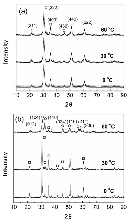
Figure 2. XRD patterns of ITO nanoparticles that were prepared by annealing of ITO precursors at 400 °C shown in Figure 1: (a) precipitated at pH 12 and (b) at pH 8. □ and ○ represent XRD peaks of cubic and rhombohedral \text{In}_2\text{O}_3 , respectively.
