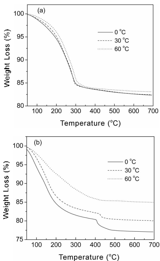
Figure 3. TGA curves of ITO precursors that were prepared at various temperatures and pH 12 (a) and 8 (b).
