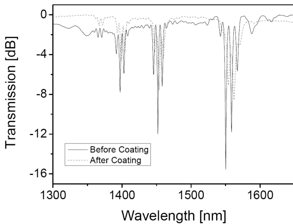
FIG. 3. Transmission spectra of an LPGP before and after palladium coating.
