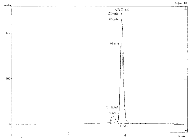
Fig. 5. HPLC-profile of the reaction products separated after 0 min, 60 min and 120 min incubation of 3-HAA with purified laccase. Retention time; 3-HAA (3.57 min), CA (3.88 min).
