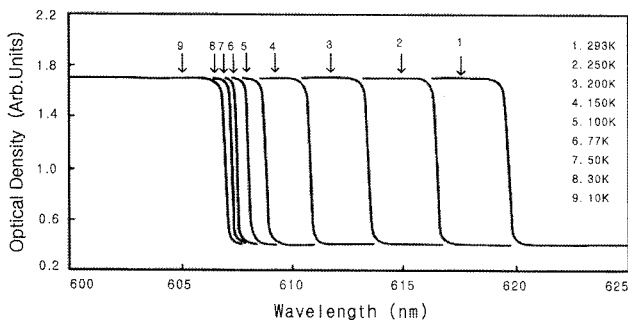
Fig. 8. Optical absorption spectra according to temperature variation of ZnIn 2 Se 4 single crystal thin films.
