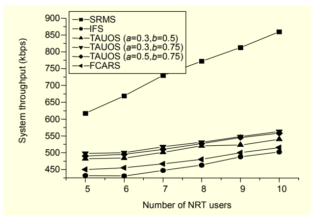
Fig. 1. System throughput.
