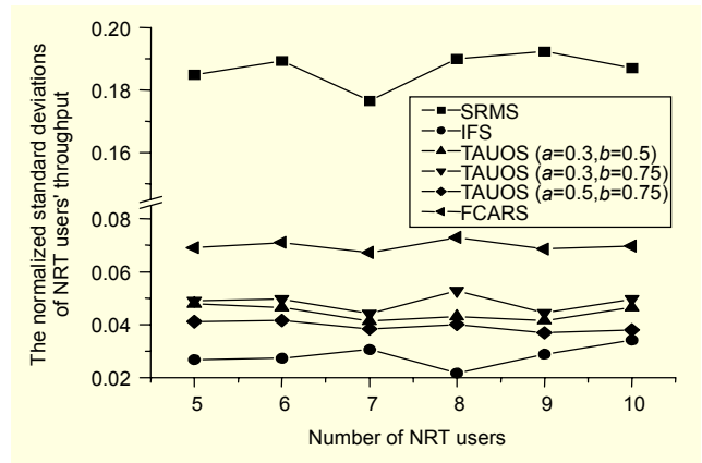
Fig. 2. The normalized standard deviations of NRT users' throughput.
