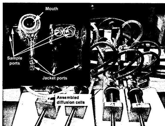
Fig. 1. A photograph showing the structure of the components of diffusion cells and when they were assembled.
