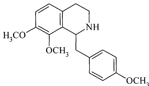
Fig. 1. Structure of Fuyuziphine.
