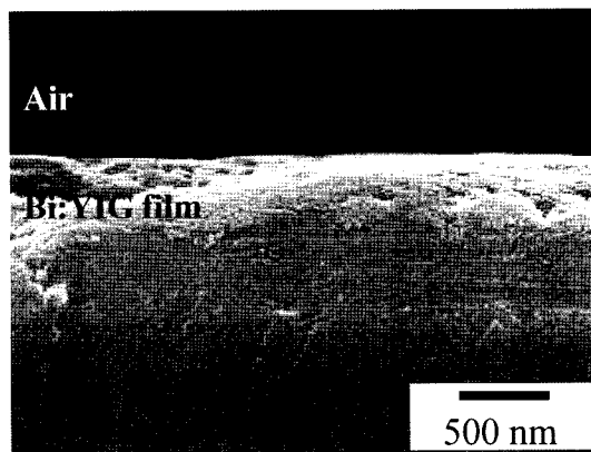
Fig. 4. SEM image of cross section of the Bi:YIG film deposited by ADM apparatus.
