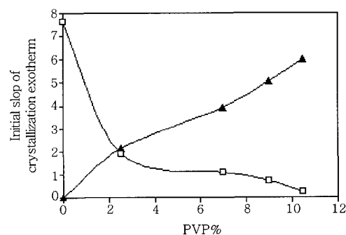
Figure 4. S_1 ( \square ) and S_2 ( \blacktriangle ) vs PVP%.
