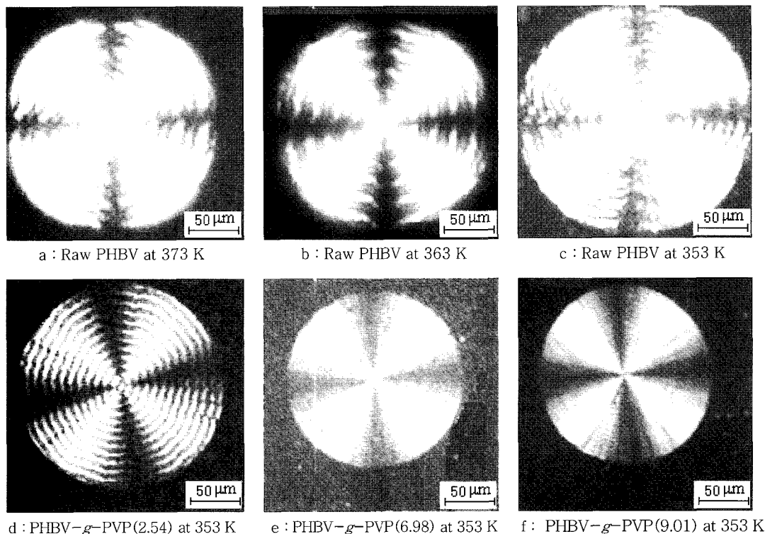
Figure 7. A series of polarized optical micrographs for samples isothermally crystallized at different temperatures.
