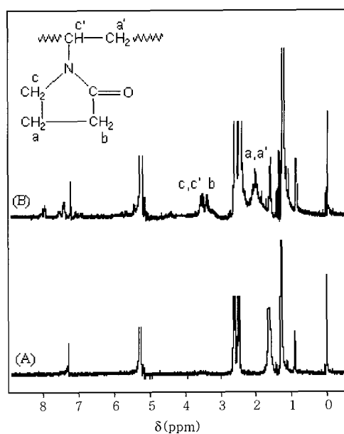
Figure 1. 1 H-NMR spectra of raw PHBV (A) and grafted PHBV with PVP% of 6.98% (B).
