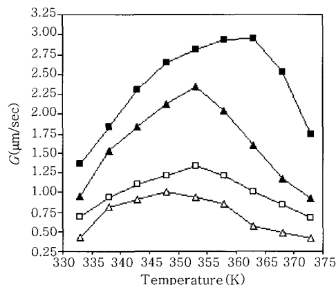
Figure 6. Spherulitic growth rate ( G ) as a function of T_c for raw PHBV and Grafted PHBV. \blacksquare Raw PHBV, \blacktriangle PHBV-g-PVP(2.54), \square PHBV-g-PVP(6.98), \triangle PHBV-g-PVP(9.01).
