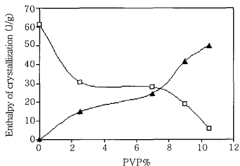
Figure 5. -\Delta H_{cc} ( \square ) and -\Delta H_{ch} ( \blacktriangle ) vs PVP%.
