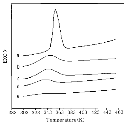
Figure 2. DSC traces of raw PHBV and grafted PHBV with different PVP% crystallized from the melt at a cooling rate of 10 K/min. (a) raw PHBV, (b) PHBV- g -PVP(2.54), (c) PHBV- g -PVP(6.98), (d) PHBV- g -PVP(9.01), and (e) PHBV- g -PVP(10.48).
