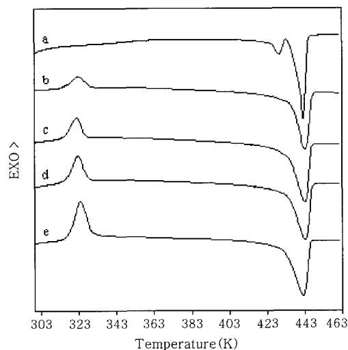
Figure 3. DSC traces of raw PHBV and grafted PHBV with different PVP% at a heating rate of 10 K/min. (a) raw PHBV, (b) PHBV- g -PVP(2.54), (c) PHBV- g -PVP(6.98), (d) PHBV- g -PVP(9.01), and (e) PHBV- g -PVP(10.48).
