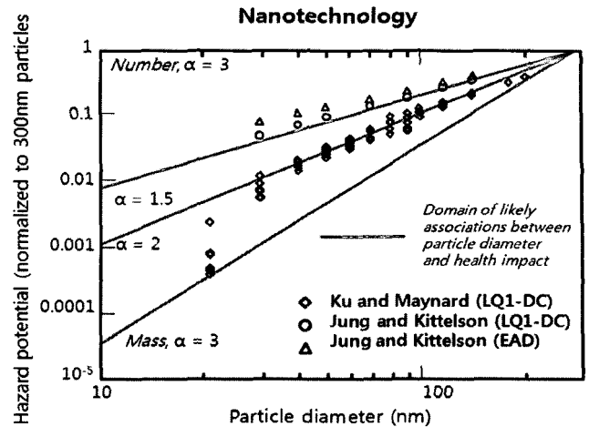
Figure 4. Possible instrument responses as a function of particle size, for evaluating exposure against airborne engineered nanomaterials [7].
