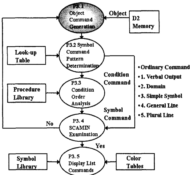
Fig. 4 Development Algorithm
