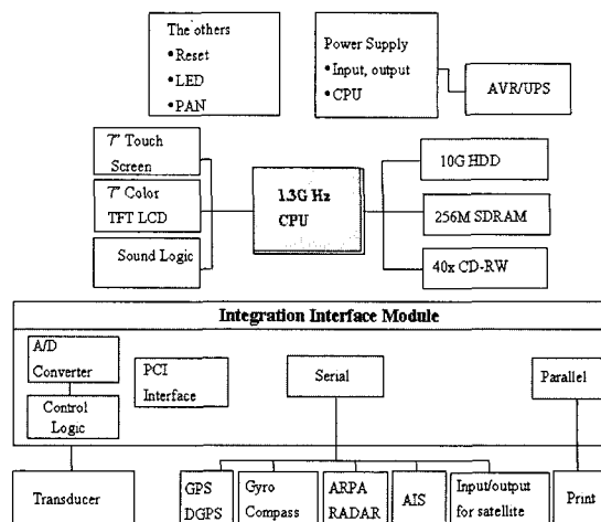
Fig. 3 s-INS Hardware Configuration
