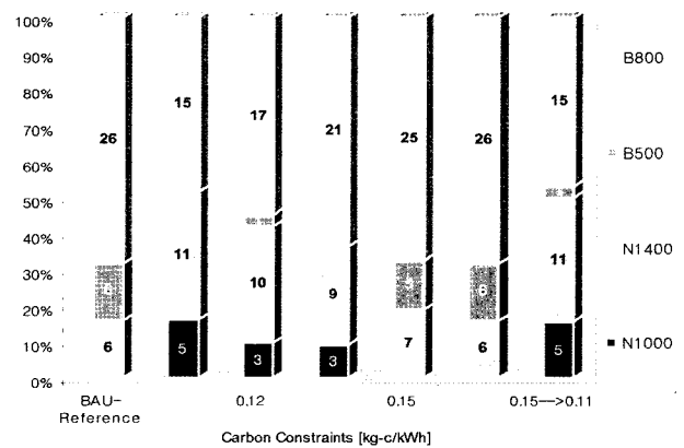
Fig. 9. Fuel Mix Changes with Respect to Various CO 2 Limits
