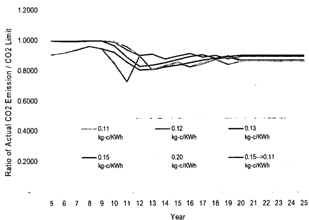
Fig.11. Changes of CO 2 Emission Margin
