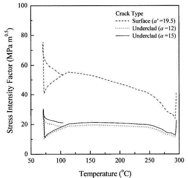
Fig. 8. Comparison of Stress Intensity Factors between Defect Types
