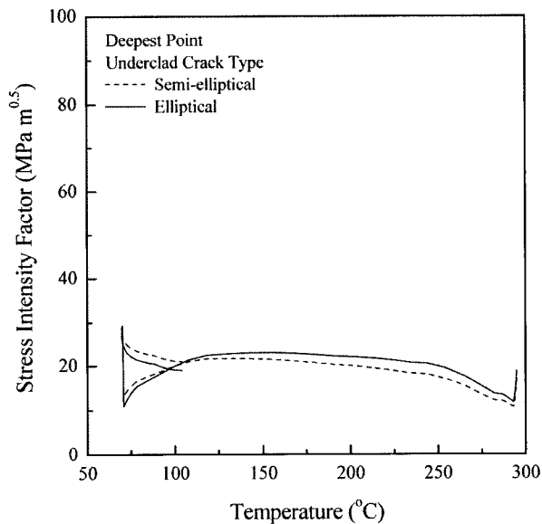
Fig. 13. Comparison of Stress Intensity Factors between Underclad Crack Shapes
