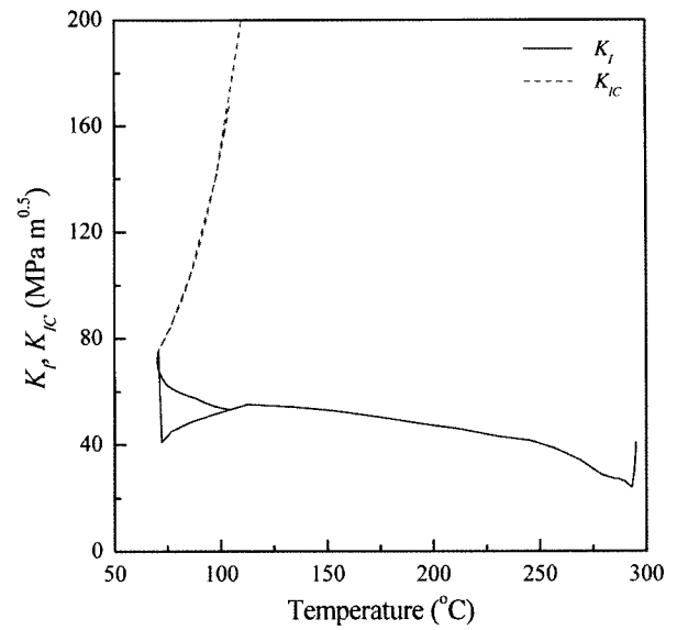
Fig. 7. Determination of Allowable RT_{NDT}
