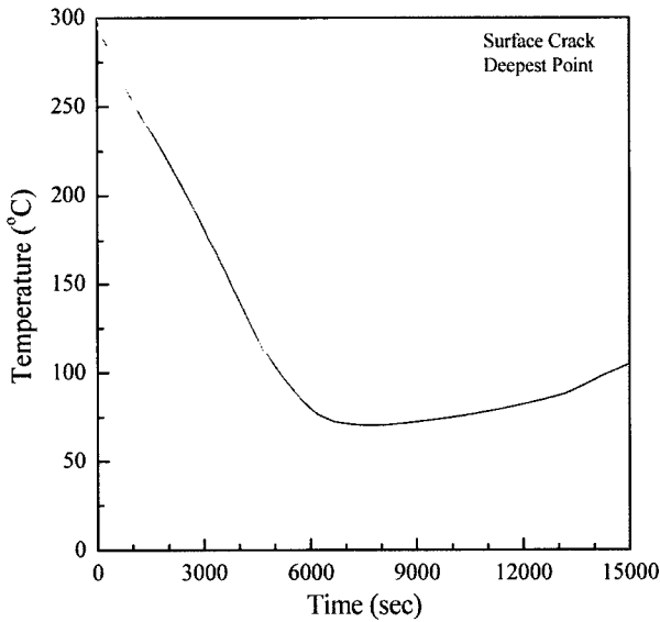
Fig. 6. Temperature at the Deepest Point
