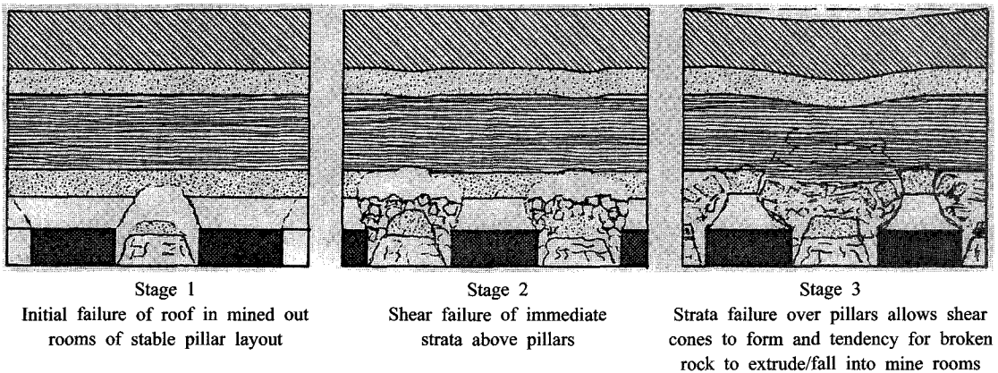
Fig. 1. Development of general surface subsidence depression over abandoned room and pillar mine workings (Whittaker and Reddish, 1989)
