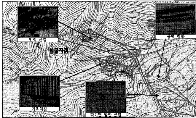
Fig. 7. Cases of surface damaged by subsidence in the abandoned metal mine
