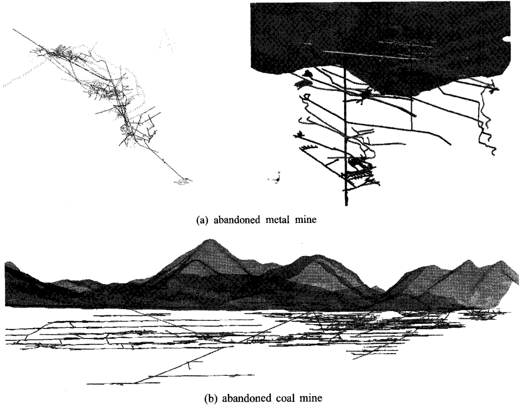
Fig. 5. Digital reconstruction of 3-D gangway networks
