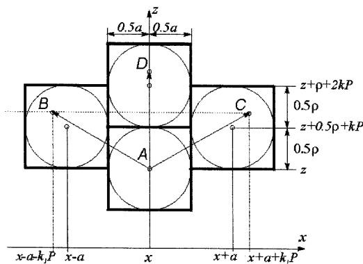
Fig. 3. Diagram of stochastic model for probabilistic displacement
