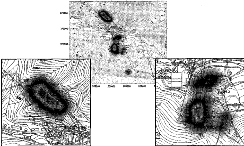
Fig. 8. Demonstration of detailed subsidence hazard map
