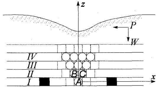
Fig. 2. Conceptual figure for stochastic model of mining subsidence
