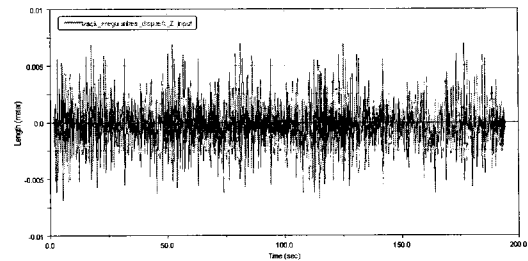
Fig. 6. Vertical irregularities of a rail profile
