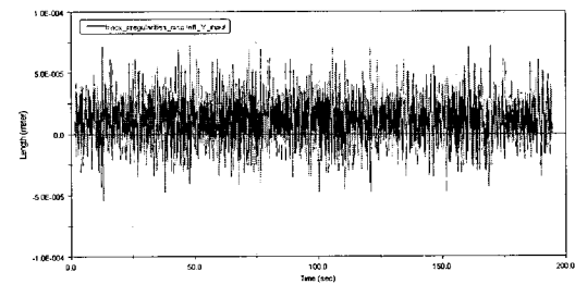
Fig. 7. Lateral irregularities of a rail profile
