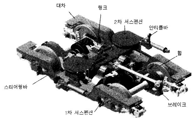
Fig. 3. A driving motor bogie
