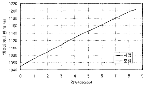
Fig. 11. Comparison of Stroke distance of a actuator between a experiment and simulation model
