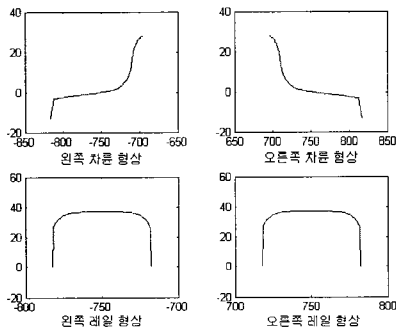
Fig. 4. Cross sectional shape of a rail and a wheel
