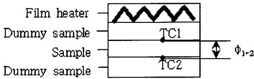
Fig. 3 Sample Configuration of Thermal Diffusivity Measurement.
