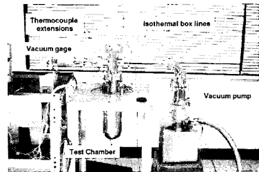
Fig. 6 Measurement System.
