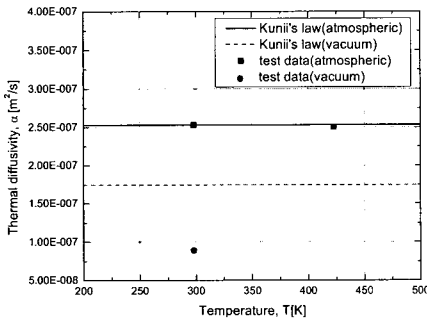
Fig. 9 Comparison of Test Results and Calculated Results.
