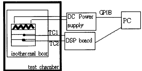
Fig. 5 Schematic Diagram of Measurement Device.
