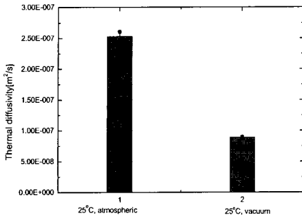
Fig. 8 Thermal Diffusivities of SP#2.
