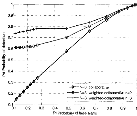
Fig. 8 ROC curves of collaborative sensing vs. weighted-collaborative sensing under Rayleigh fading with slow fading environment
