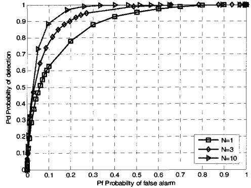
Fig. 3 ROC curves of collaborative sensing under AWGN
