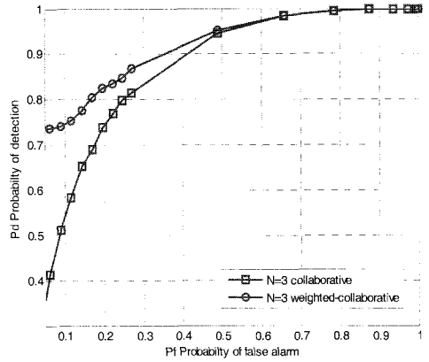
Fig. 10 ROC curves of collaborative sensing vs. weighted-collaborative sensing under AWGN with fast fading environment
