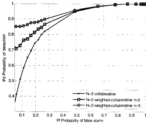
Fig. 7 ROC curves of collaborative sensing vs. weighted-collaborative sensing under AWGN with slow fading environment
