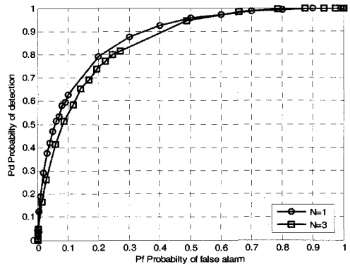
Fig. 4 ROC curves of collaborative sensing vs. best local sensing under AWGN
