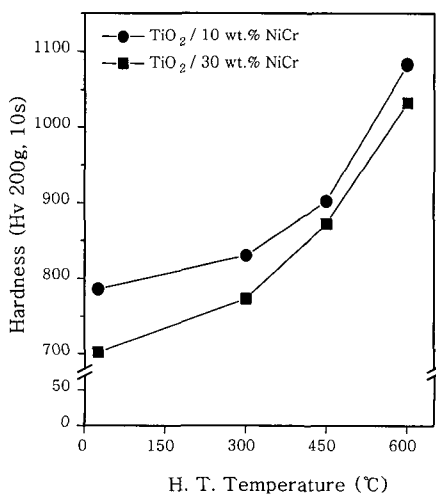
Fig. 11 Hardness of TiO 2 -NiCr heating coatings according to as-sprayed and heat treated temperatures
