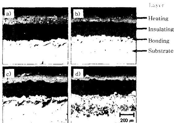
Fig. 5 Cross sectional optical images of TiO 2 -10wt.% NiCr of plasma sprayed coating layers at heat treated temperatures a) as-sprayed, b) 300 °C, c) 450 °C, d) 600 °C
