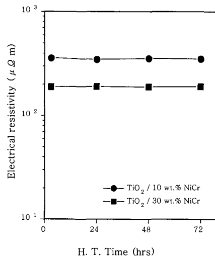
Fig. 13 Electrical specific resistivity of heating coatings on heat treated times at 300℃
