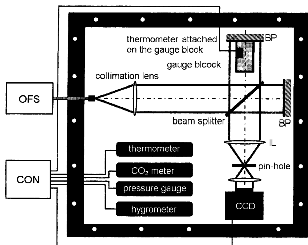
Fig. 2 Optical configuration of the gauge block interferometer (OFS: optical frequency synthesizer, CON: controller, BP: base plate, IL: imaging lens)
