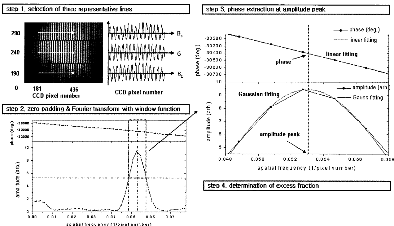
Fig. 3 Fourier transform fringe analysis used to determine the excessive fraction
