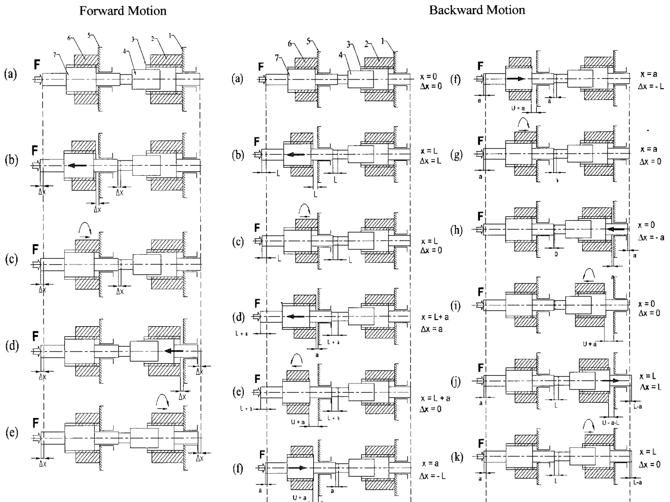
Fig. 3 Operation of forward motion and Backward Motion (Input support(1), Input feeding screw(2), Input shaft (3), Piezoelectric actuator (4), Output support (5), Output feeding screw (6), Output shaft (7)). In backward motion schematic, x represents the extension of actuator and \Delta x represents the increment in the extension
