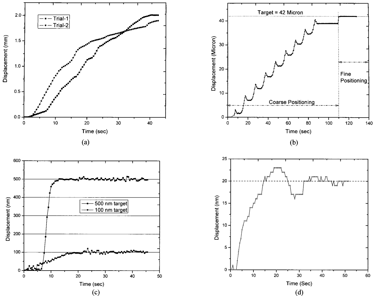
Fig. 8 Performance of nanopositioner a) Long range positioning b) Hybrid positioning c) Fine positioning d) Minimum resolution performance
