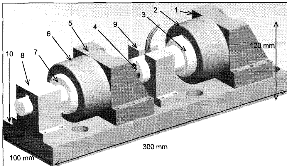
Fig. 2 Geometric model of Nanopositioner (Base (10), Supports (1, 5, 8, 9), Feeding screws (6, 2), Input and Output Shaft (7, 3), Actuator assembly (4)). Stepper motor assembly connecting the feeding screws is not shown in the figure
