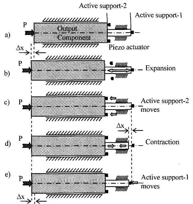
Fig. 1 Mechanism of the actuator
