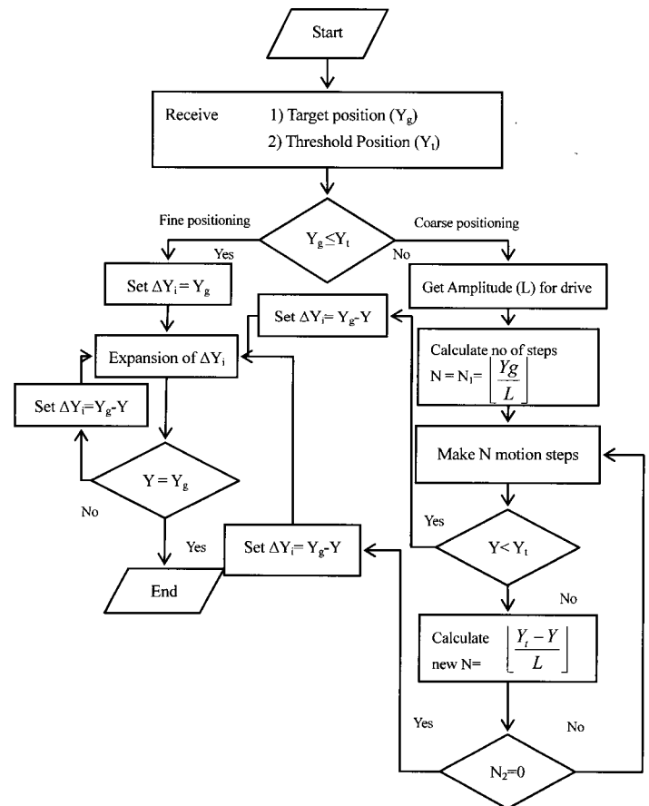
Fig. 5 Algorithm used for dual positioning (Y is the position variable)
