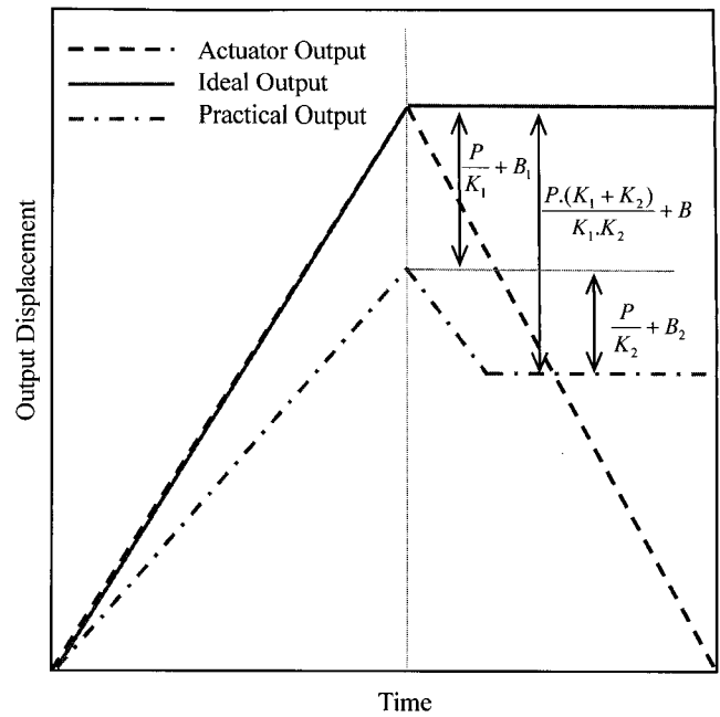
Fig. 4 Ideal output , actuator output and practical output in one step motion
