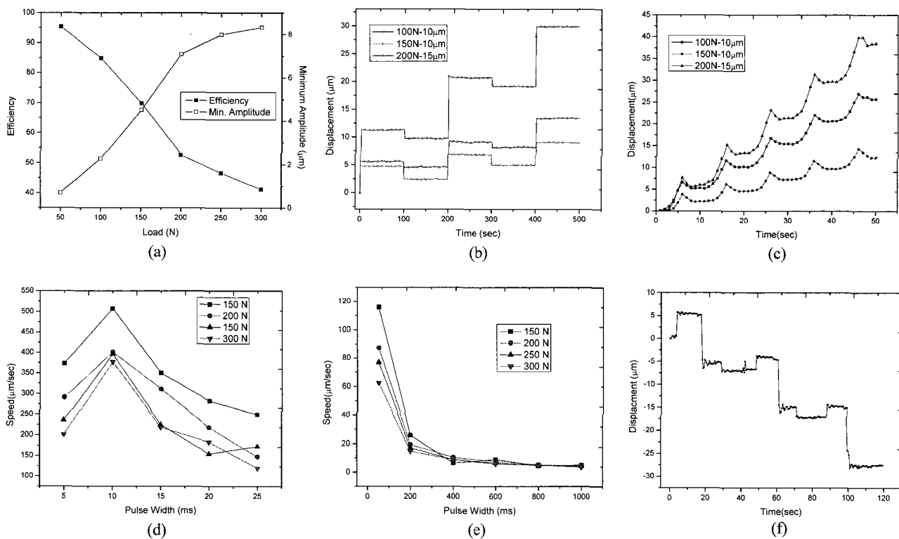
Fig. 7 Performance of nanopositioner a) efficiency and minimum displacement for the nanopositioner b) forward motion with a square signal c) forward motion with a triangle signal d) dynamic performance with short pulse width e) dynamic performance with long pulse width f) backward motion of the nanopositioner
