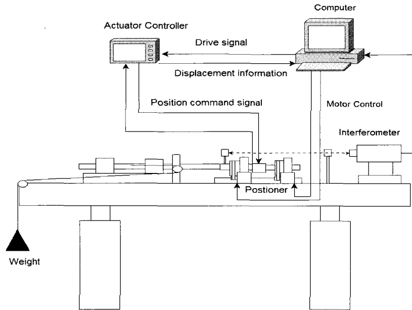
Fig. 6 Experimental setup of the nanopositioner
