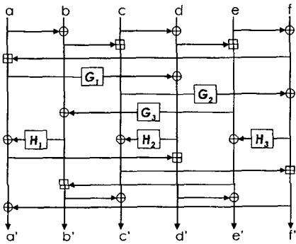
Figure 3: State Update Function ( F Function).
