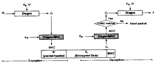
Figure 6: Authenticated encryption process flow.
