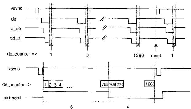
Fig. 5. Generating blinking signal using de signal counting.
