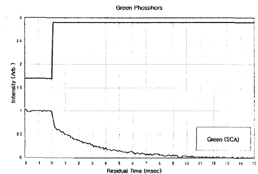
(b) Residual time of green phosphor
