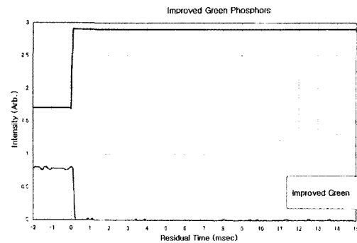
(b) Result of residual time of improved green phosphor
