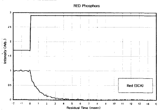
(a) Residual time of red phosphor
