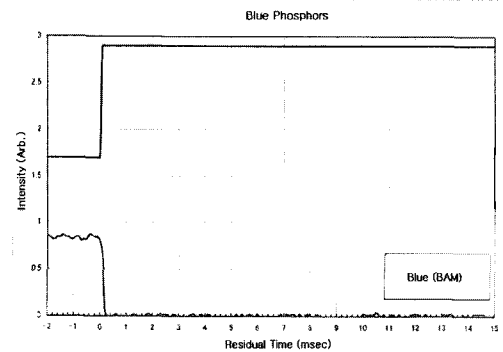
(c) Residual time of blue phosphor
