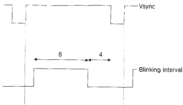
Fig. 4. Generating blinking signal using Vsync signal.
