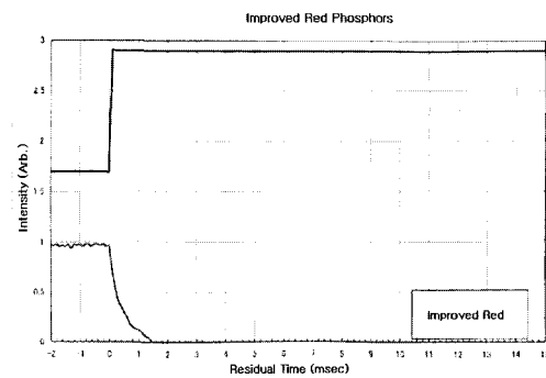
(a) Residual time of improved red phosphor
