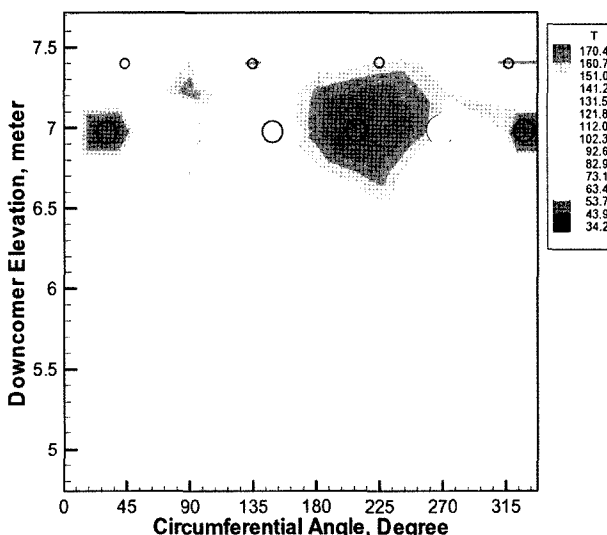
Fig. 3. Isothermal Line Showing Multi-Dimensional Phenomena in the Downcomer: DVI-2&4 Injection Case
