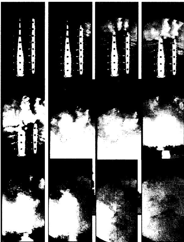
Fig. 15. Blowdown Process Observed in the B&C Facility with a Prototypic Sparger
