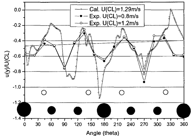
Fig. 12. Typical Results of Velocity Information in the RPV Downcomer: BOMIX-II Test vs. CFD Analysis
