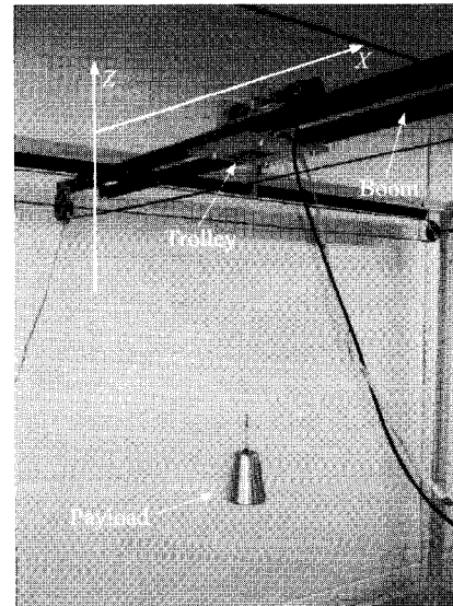
Fig. 2. The 3D pilot crane used in experiment.
