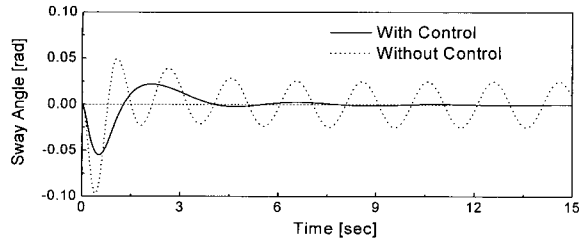
Fig. 3. Comparison of the sway angles with and without control, that is, f=0 in (16).
