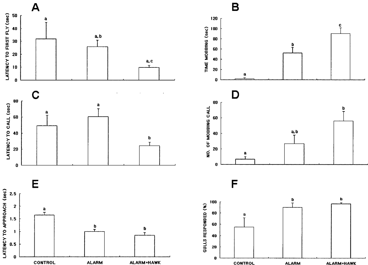
Fig. 4. Behavioral responses of gull flocks during the post-breeding period to mew calls (control), alarm calls only, and alarm calls with a stuffed hawk. Bar represent mean \pm SE. Significant differences among the three experimental treatments were detected for all six response variables; the use of the same superscript letter indicates means that were not significantly different in post-hoc pair-wise comparisons (Tukey test, p>0.05 ).
