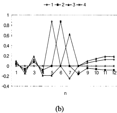
Fig. 3. Impulse responses for the denoising system (DCT to DCT domain) (b) Proposed system 2
