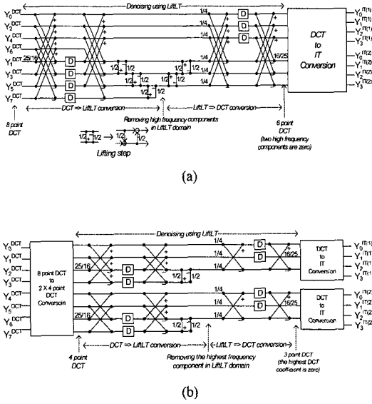
Fig. 2. Denoising in the LiftLT domain (a) Proposed system 1 (b) Proposed system 2
