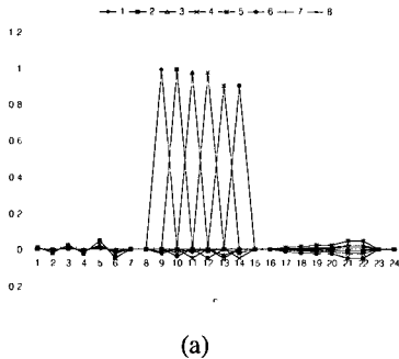
Fig. 3. Impulse responses for the denoising system (DCT to DCT domain) (a) Proposed system 1
