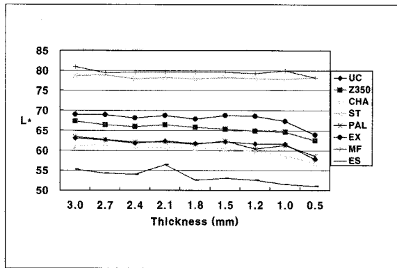
Figure 1. Shifts of L* values on the Mustard background according to the thickness. Abbreviation. UC: Universal composite, Z350: Filtek Z350, CHA: Charisma, ST: Clearfil ST, PAL: Palpaque Estelite, EX: Esthet-X, MF: Metafil Flo, ES: Estelite Sigma.
