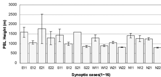
Fig. 3. Distributions of mixed layer height for the sixteen synoptic classes derived from the upper sounding meteorological observations during 2001
