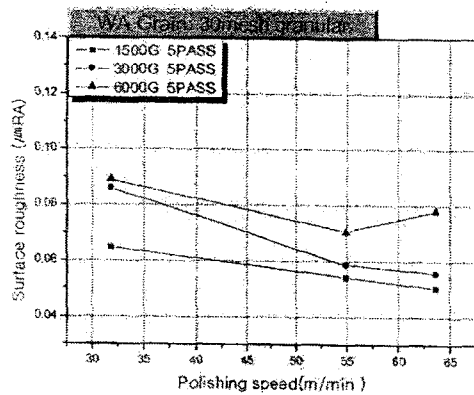
Fig.4 (a) Surface roughness according to polishing condition (granular structure type magnetic abrasive: WA)
