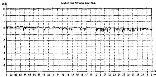
Fig. 3A surface roughness curve of internal face of seamless stainless steel tube.
