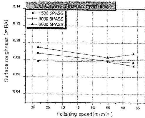
Fig. 4 (a) Surface roughness according to polishing condition (granular structure type magnetic abrasive: GC)
