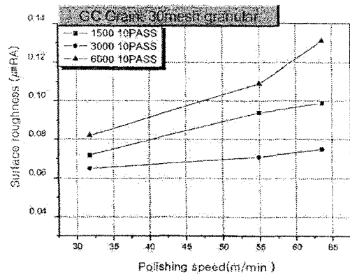
Fig. 4 (b) Surface roughness according to polishing condition (granular structure type magnetic abrasive: GC)
