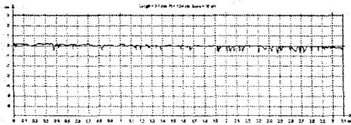
Fig. 3A surface roughness curve of internal face inseamlrss stainless steel tube.
