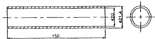
Fig. 2 Geometry and dimension of specimen
