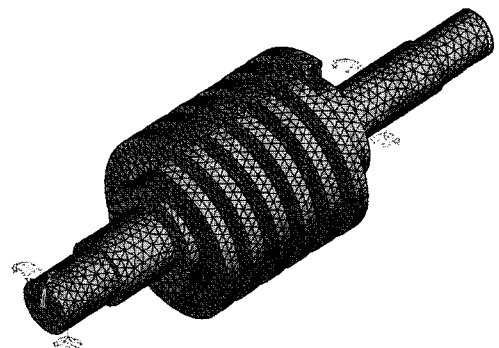
Fig. 3 3-D FE model of X screw rotor excluding lobe
