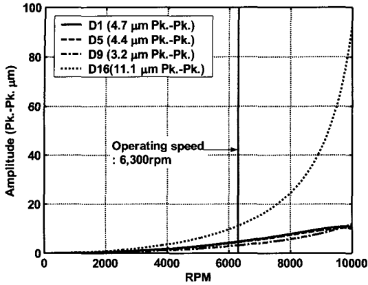
Fig. 19 Unbalance response of Y screw rotor for Case II
