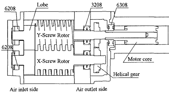
Fig. 1 Schematic drawing of screw rotors of the dry vacuum pump
