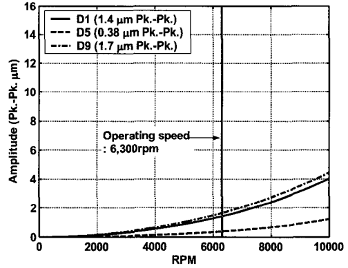
Fig. 17 Unbalance response of X screw rotor for Case III
