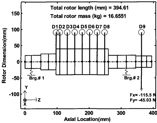
Fig. 5 Full FE model of X screw rotor including lobe & gear (D1~D9 : Equivalent concentrated mass & inertia)
