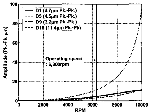
Fig. 18 Unbalance response of Y screw rotor for Case I
