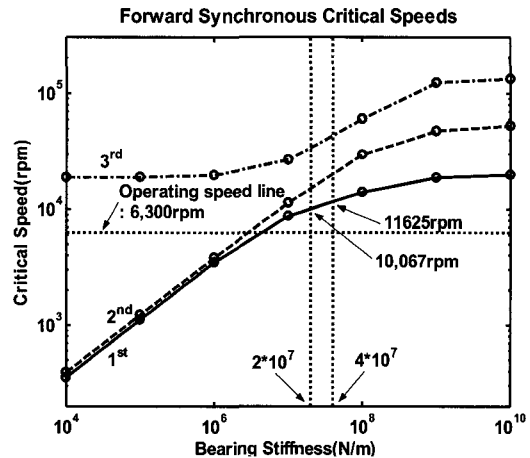
Fig. 10 Forward synchronous critical speeds for Y screw rotor
