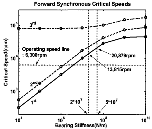
Fig. 9 Forward synchronous critical speeds for X screw rotor
