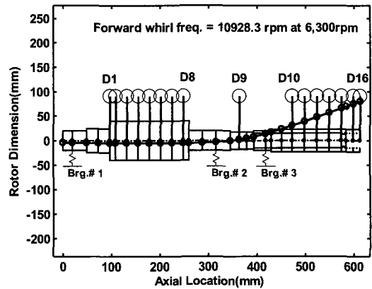
Fig. 14 1 st mode shape of the Y rotor-bearing system
