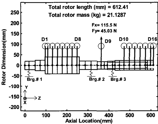
Fig. 6 Full FE model of Y screw rotor including lobe & gear (D1~D16 : Equivalent concentrated mass & inertia)
