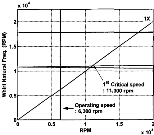
Fig. 12 Campbell diagram of the Y rotor-bearing system
