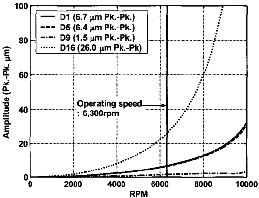
Fig. 20 Unbalance response of Y screw rotor for Case III
