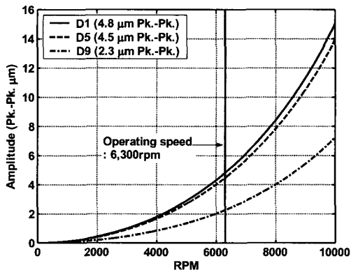
Fig. 16 Unbalance response of X screw rotor for Case II
