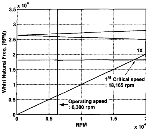
Fig. 11 Campbell diagram of the X rotor-bearing system
