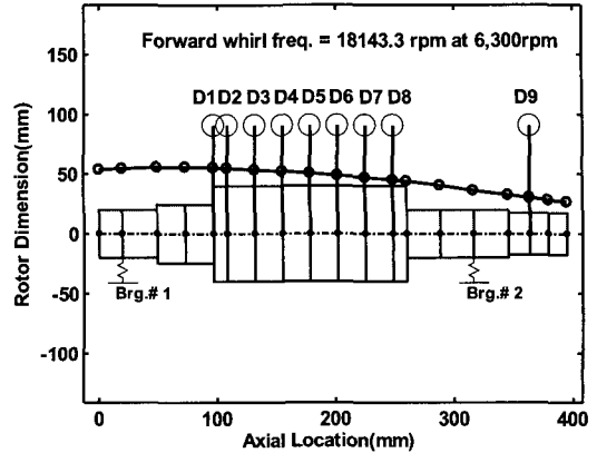
Fig. 13 1 st mode shape of the X rotor-bearing system
