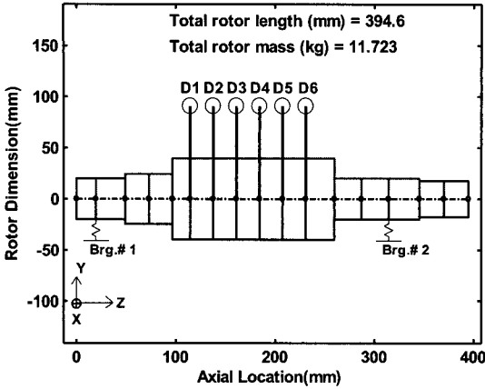
Fig. 4 Rotordynamic FE model of X rotor excluding lobe (D1~D6 : Equivalent concentrated mass & inertia)
