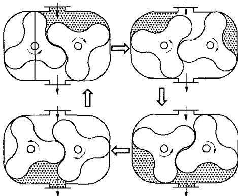
Fig. 2 Operation principle of air picking
