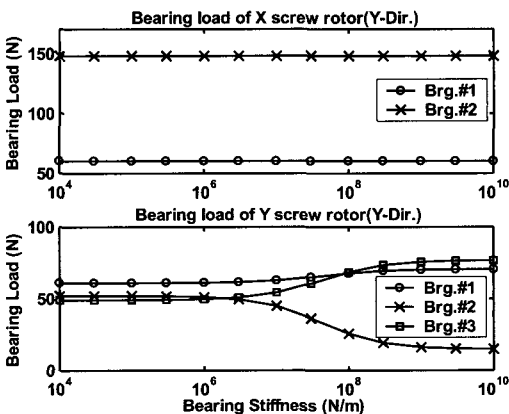
Fig. 7 Bearing loads as a function of bearing stiffness
