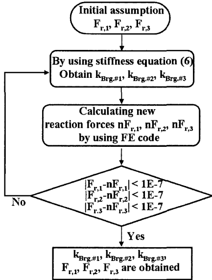
Fig. 8 Calculation diagram of bearing load, where
