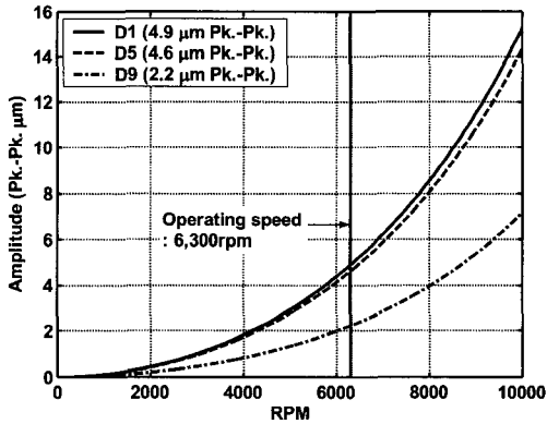
Fig. 15 Unbalance response of X screw rotor for Case I
