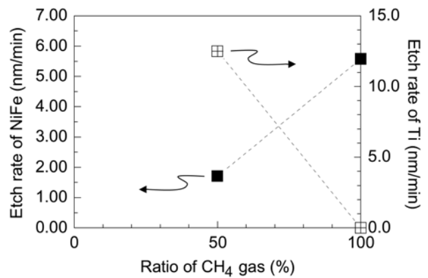
Fig. 3. Etch rate of NiFe and that of the Ti mask as a function of the ratio of \text{CH}_4 gas. The etching was carried out under the ICP source power of 500 W and the \text{O}_2 gas flow of 10 SCCM.
