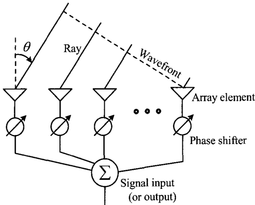
Fig. 1 Typical phased array antenna.
