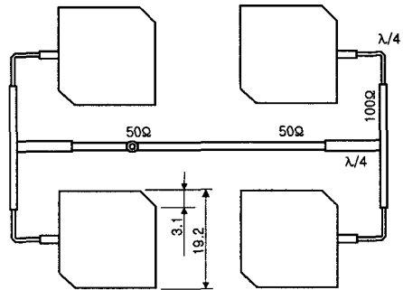
(b) Radiator
