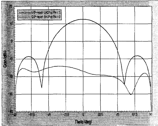
(a) E-plane
